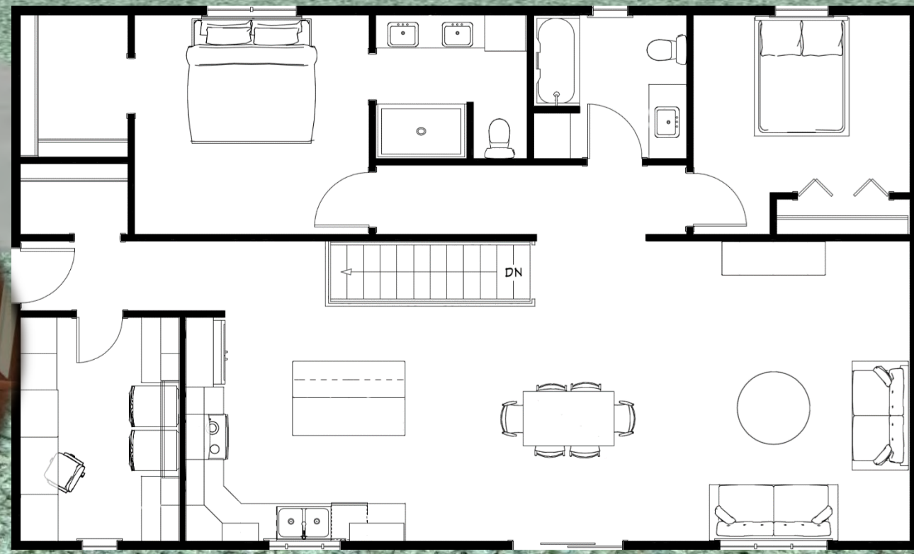
Redwood: 30'x50' – 1460sf – 2Beds/2Baths
